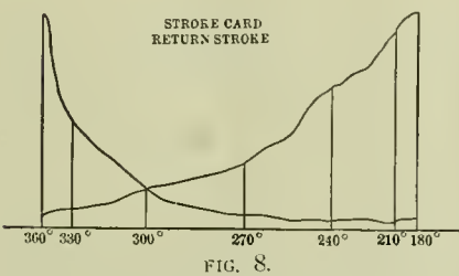
FIGS. 7 AND 8.—STROKE CARDS FOR THE INDICATOR CARD SHOWN IN FIG. 6.
